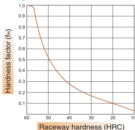
Fig. 2 Hardness factor
