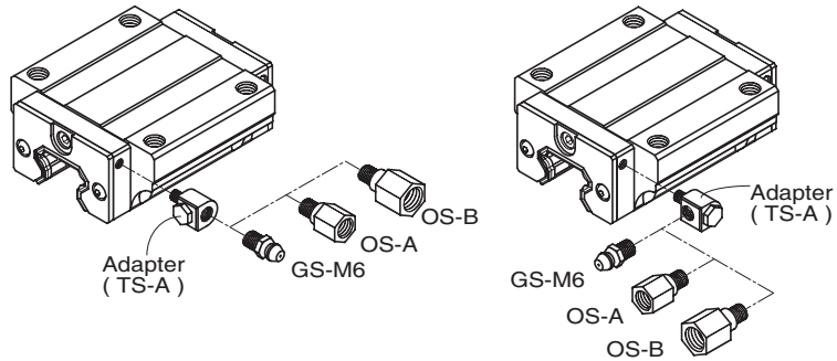
Fig. 12 Lateral usage
