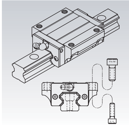
MSA-E Type
