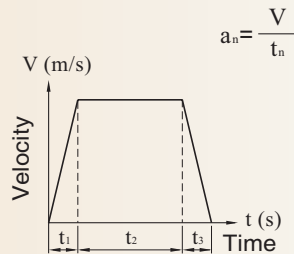
Velocity diagram
