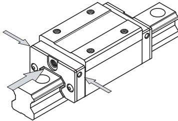
Fig. 11 Lubrication location
