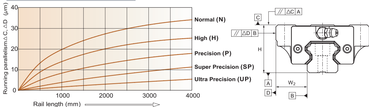
Fig.15 Running Parallelism of Carriage
