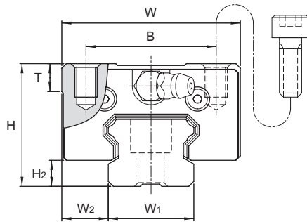
MSB-S / MSB-LS
