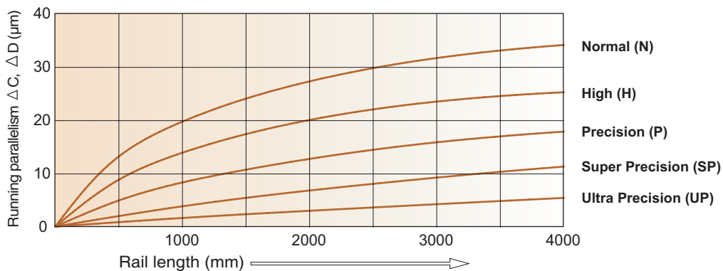
Fig.17 Running Parallelism of Carriage
