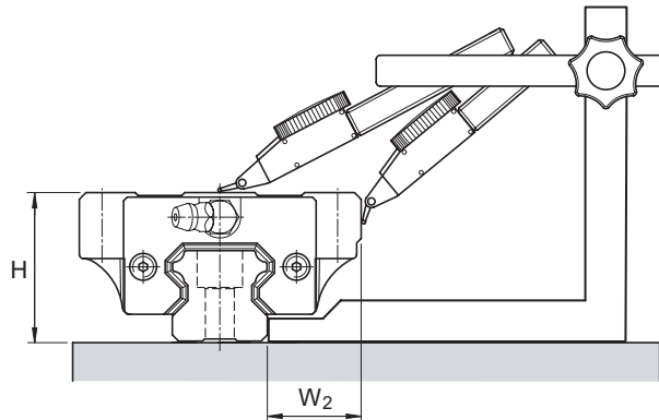
Fig. 9 Measuring the running parallelism
