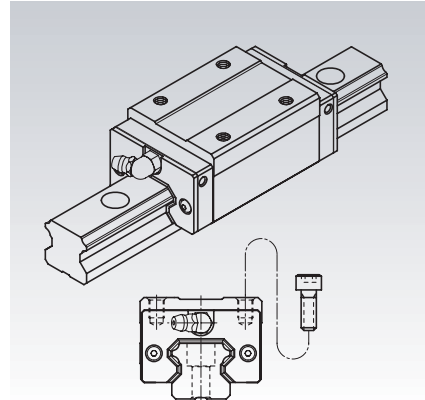
MSA-S Type
