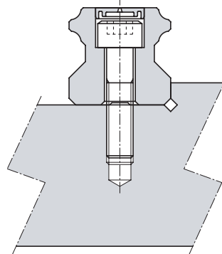
Fig.13 Plastic cap for rail mounting hole
