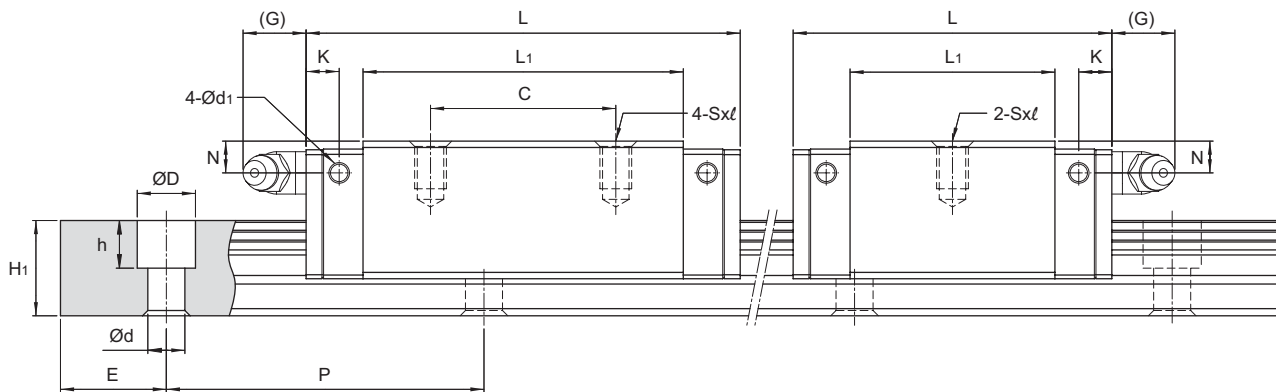
MSB-S / MSB-LS
