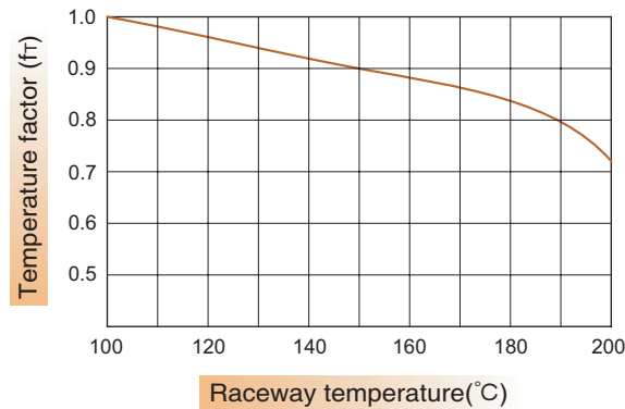
Fig. 3 Temperature factor
