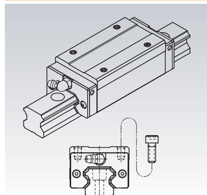
MSA-LS Type
