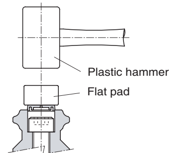
Installation method
